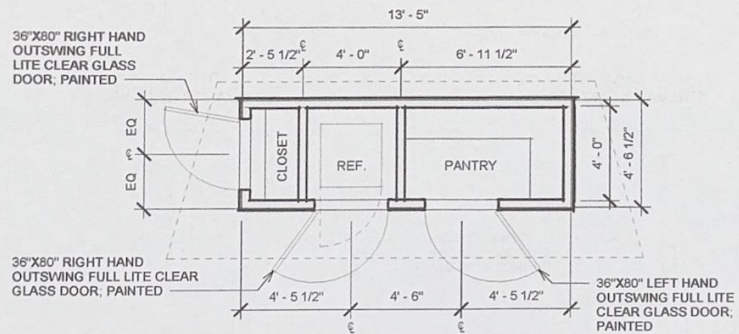
③ FLOOR PLAN 1/4" = 1'-0"
