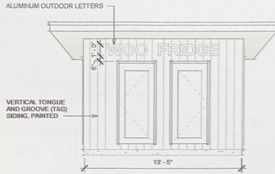
② FRONT ELEVATION 1/4" = 1'-0"
