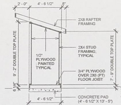
② OVERALL FRAMING DIMENSIONS 1/4" = 1'-0"
