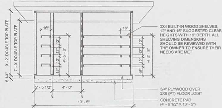
④ OVERALL FRAMING DIMENSIONS 1/4" = 1'-0"
