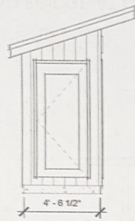
① SIDE ELEVATION 1/4" = 1'-0"
