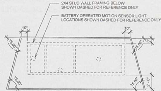
① ROOF PLAN 1/4" = 1'-0"
