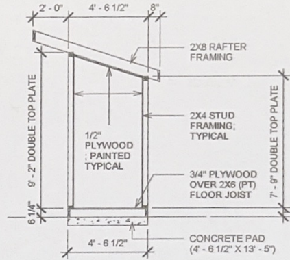
② OVERALL FRAMING DIMENSIONS 1/4" = 1'-0"
